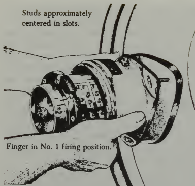
FIGURE 4-48. Distributor installation.
